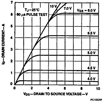
Figure 3 Transfer Characteristics
