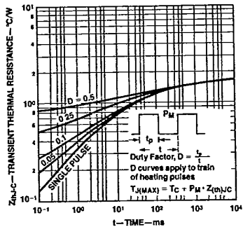
Figure 11 Transient Thermal Resistance
