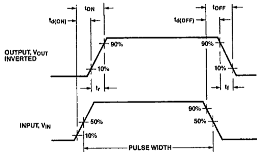
Figure 13 Switching Waveforms
